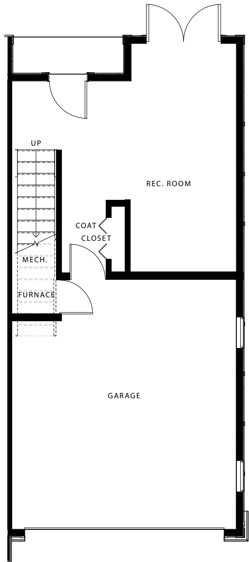
LOWER LEVEL: 334 SQ FT
