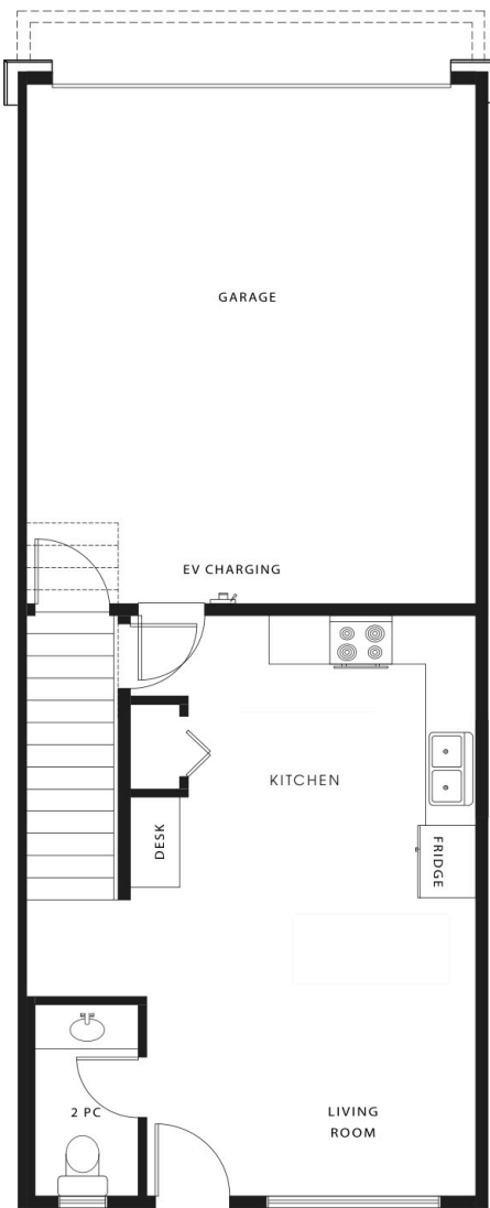
MAIN FLOOR · 463 SQ FT
